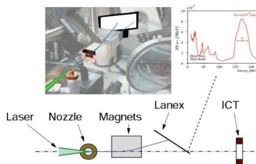
Figure 4: Experimental set-up and spectra obtained in the bubble regime.
