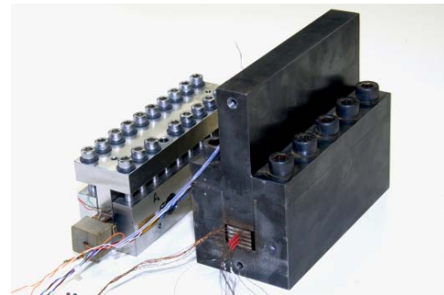
Coils stack jigs for heat transfer measurements
