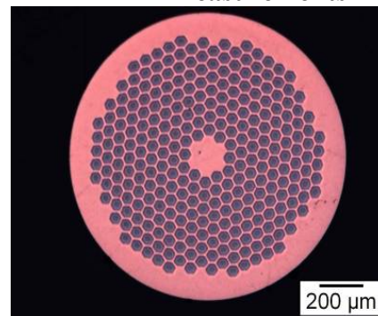
PIT strand cross section
