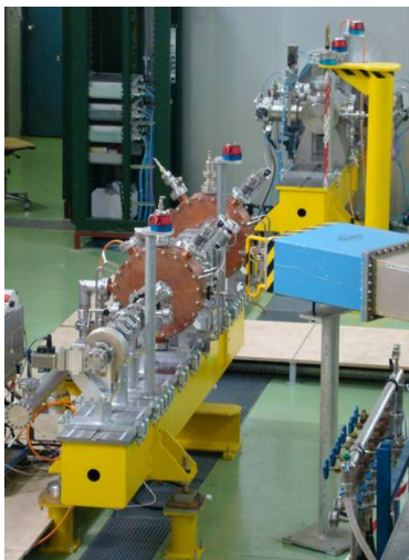
Prototypes of superconducting accelerating structures and components. From left, elliptical cavity B, spoke cavity, prototype coupler.
