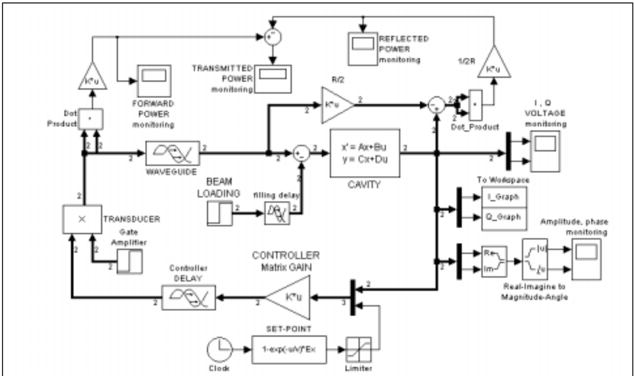
Figure 6. The state space model implementation for the cavity control system.
