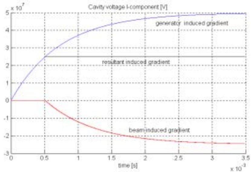
Figure 3. Cavity voltage response for step input signal and delayed beam loading current.
